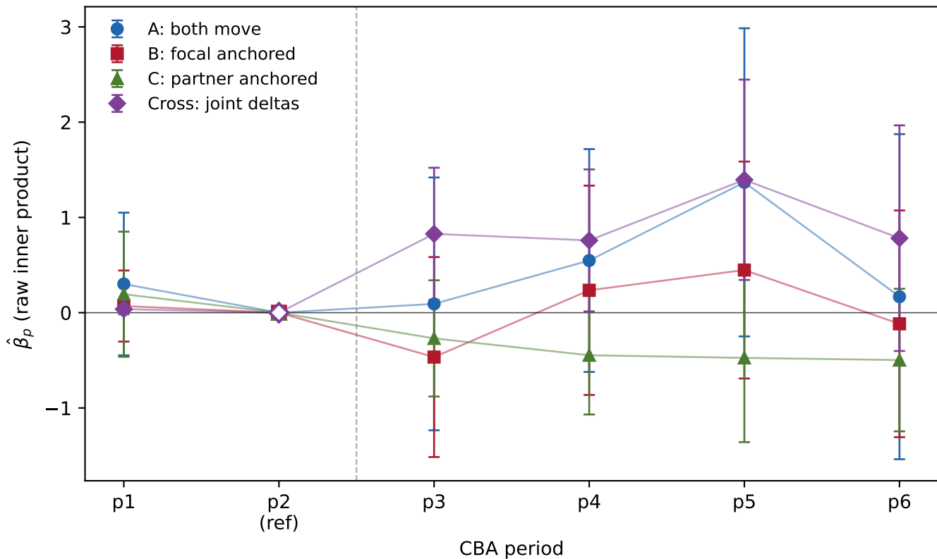
Bilinear decomposition: raw inner product
