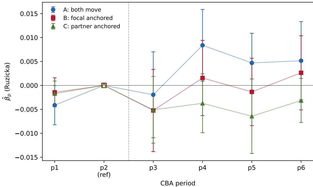
Ruzicka similarity
