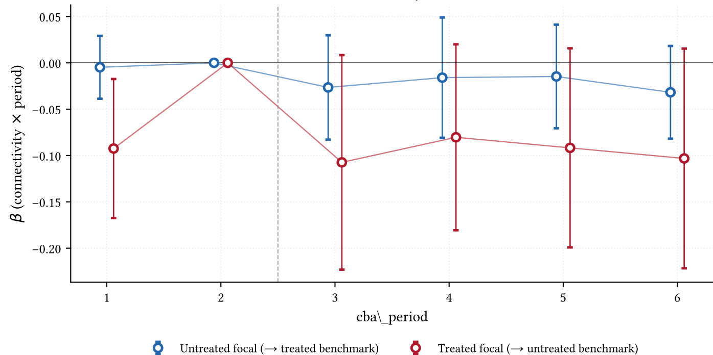
Ruzicka similarity (counts)
