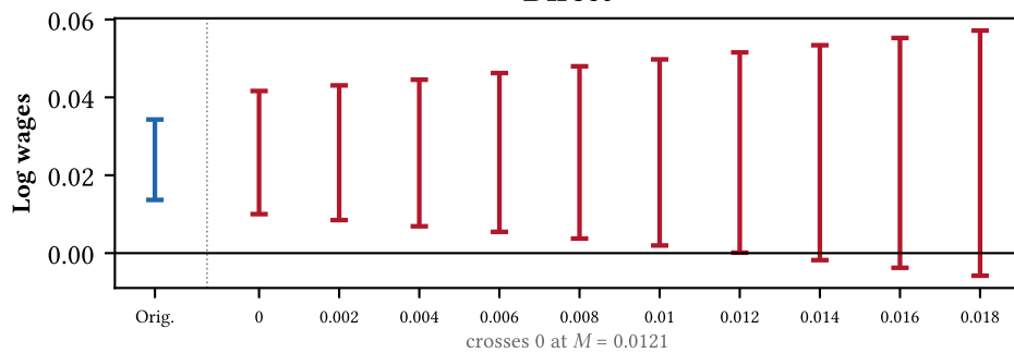
Direct
