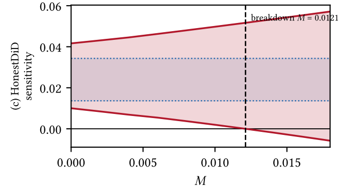
(c) Sensitivity: \Delta^{SD} (smoothness)
