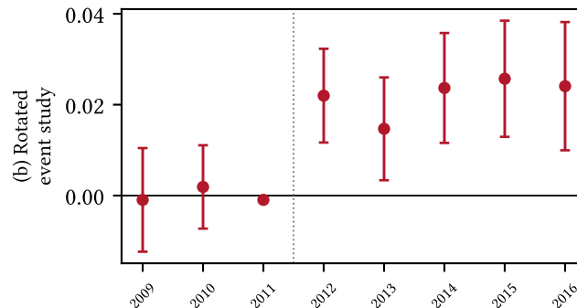
(b) Rotated (detrended) event study
