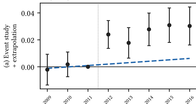
(a) Coefficients + linear extrapolation
