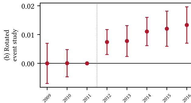
(b) Rotated (detrended) event study
