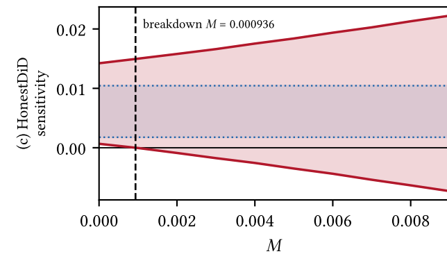
(c) Sensitivity: \Delta^{SD} (smoothness)
