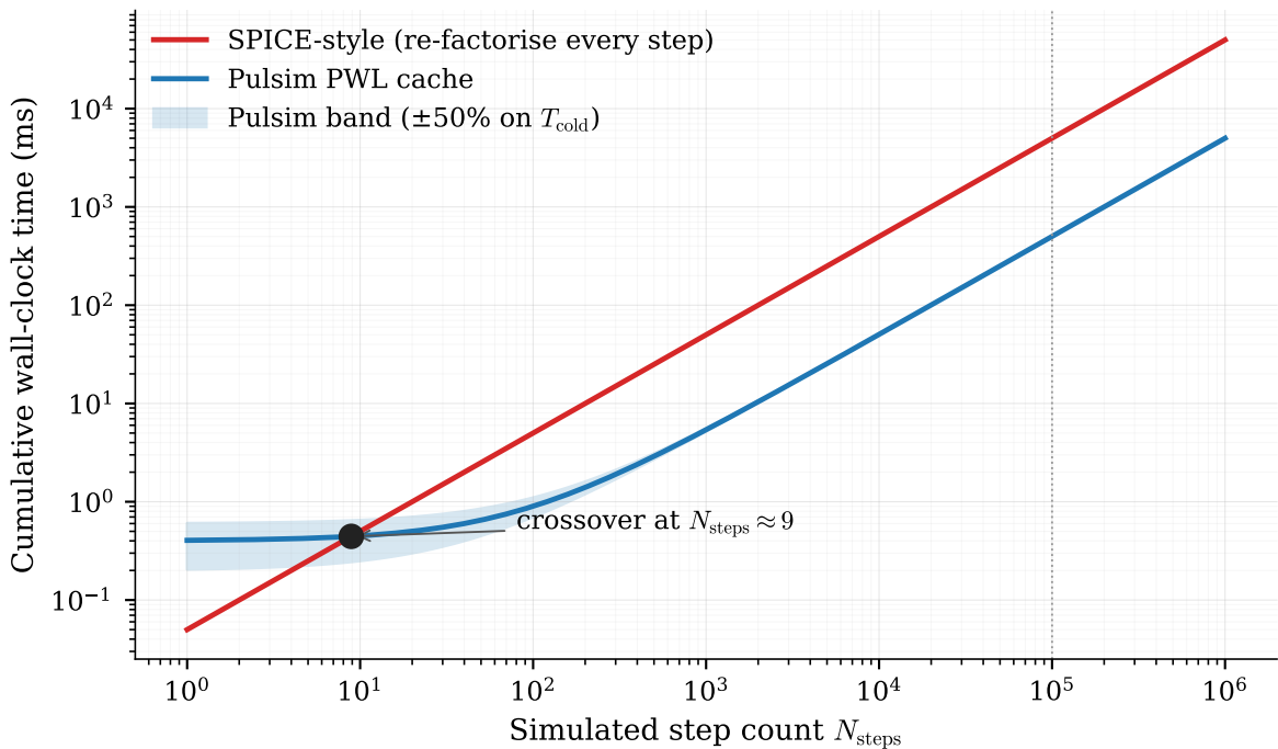
PWL cache amortisation: cumulative cost vs simulation length (per-step parameters: T_{\text{cold}} = 100\ \mu\text{s} , T_{\text{hot}} = 5\ \mu\text{s} , T_{\text{SPICE}} = 50\ \mu\text{s} , |\text{visited}| = 4 )
