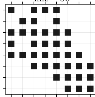
L + U , RCM ordering nnz = 38
