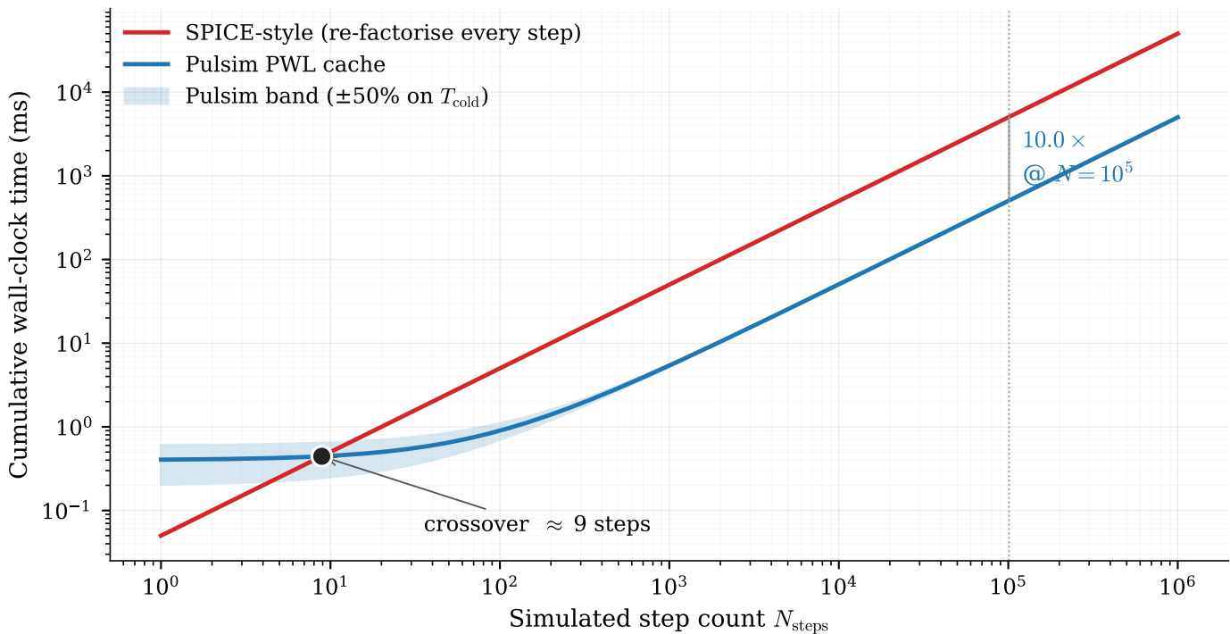
PWL cache amortisation: cumulative cost vs simulation length (per-step parameters: T_{\text{cold}} = 100\ \mu\text{s} , T_{\text{hot}} = 5\ \mu\text{s} , T_{\text{SPICE}} = 50\ \mu\text{s} , |\text{visited}| = 4 )
