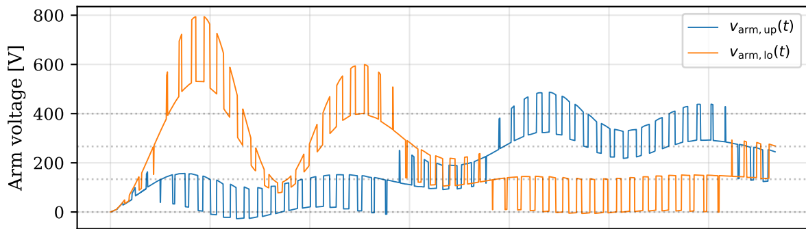
Arm voltages — 4 discrete levels at k \cdot V_C , k \in [0, 3]
