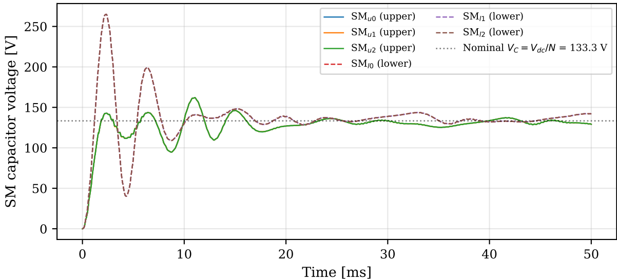
All 6 sub-module cap voltages — sort-and-select
