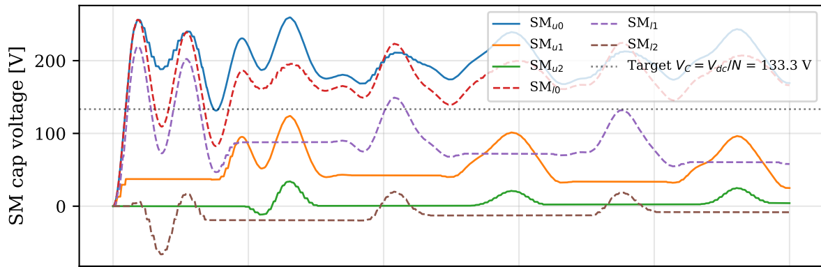
Open-loop — caps diverge in a few cycles
