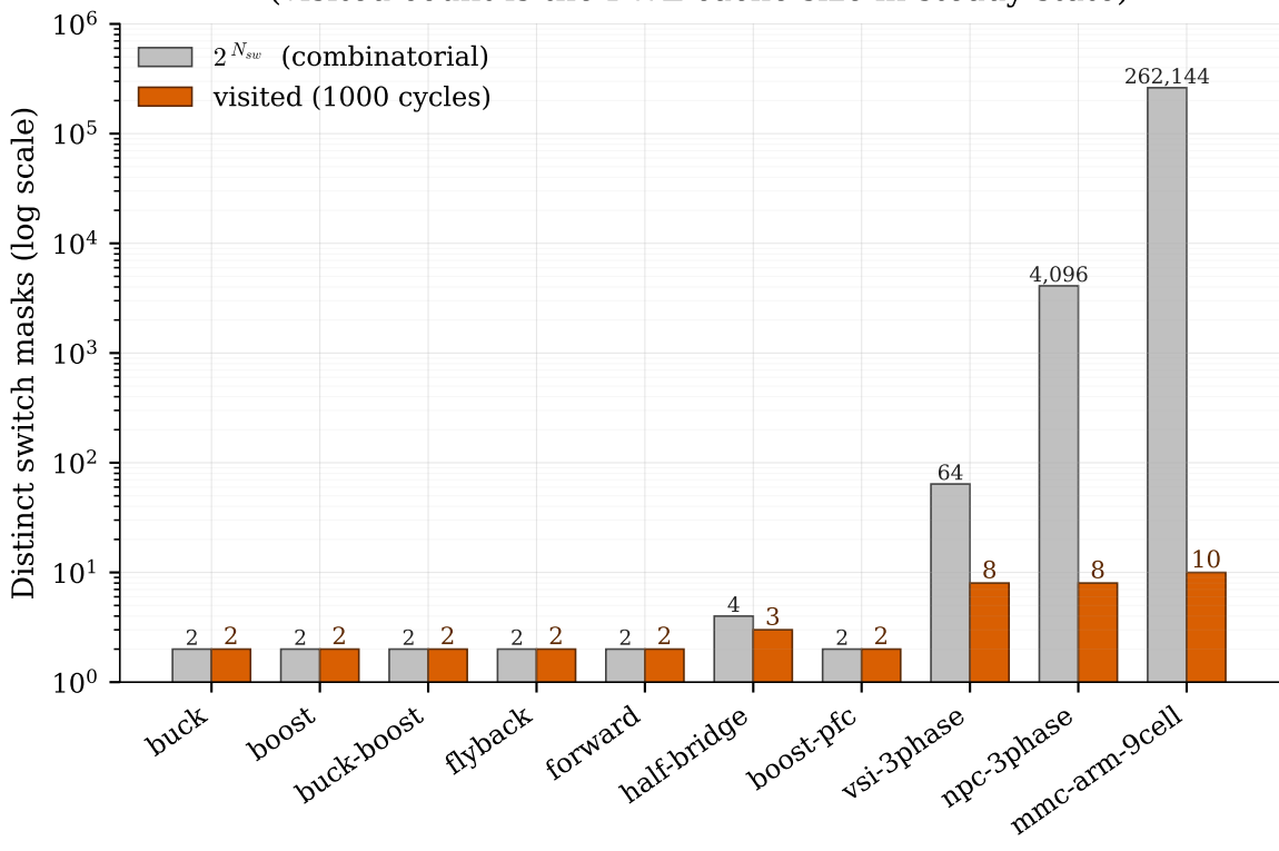
Topology census across the 10 reference Pulsim projects (visited count is the PWL-cache size in steady state)
