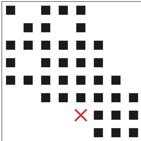
(b) Actual L + U post-pivot nnz = 38, \times = 1 entries the symbolic missed
