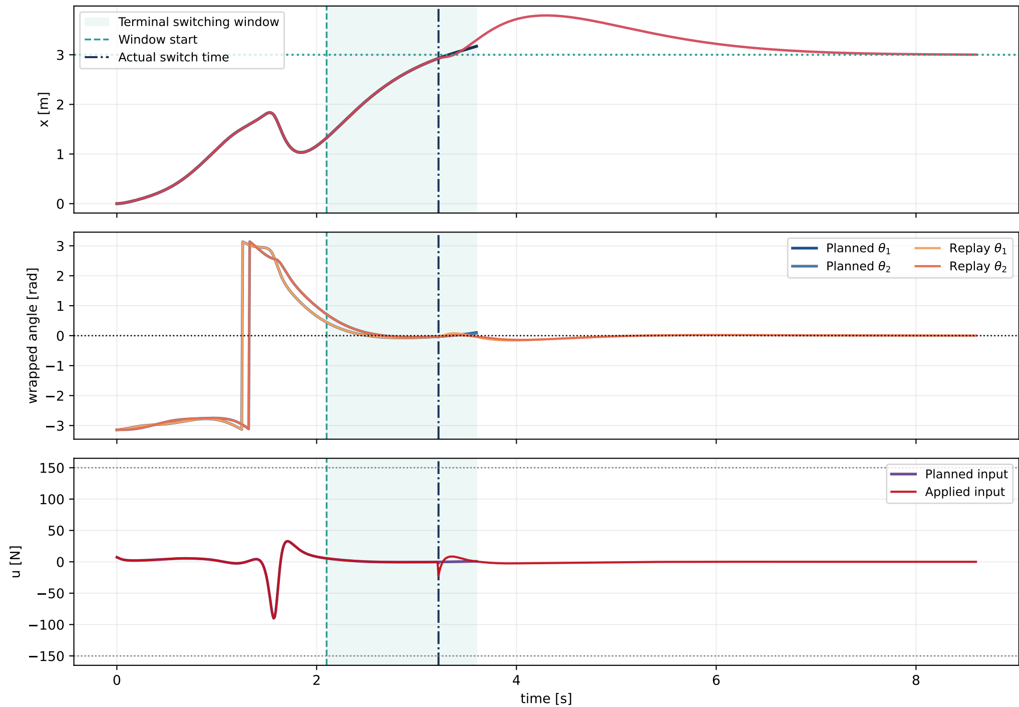
Hybrid TO + trajectory-tracking LQR + terminal equilibrium LQR replay (dt = 0.01 s, N = 360)
