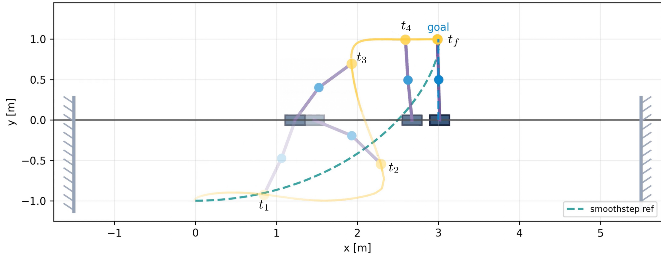
Double Inverted Pendulum Cart-Pole
