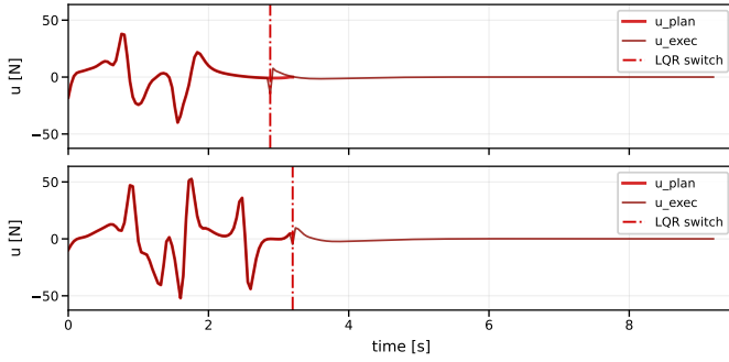
Fig. 5. Applied control forces for Scenarios 2 and 3. The force remains within the actuator bound in both cases. The obstacle-aware scenarios require different input timing because the cart motion must avoid obstacles while still arriving near the upright configuration. After the LQR switch, the input decreases as the feedback controller damps the remaining motion.
