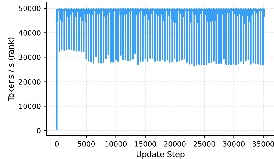
Per-Rank Throughput
