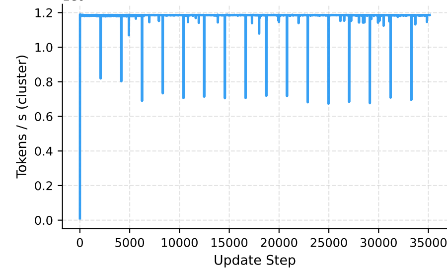
Cluster Throughput
