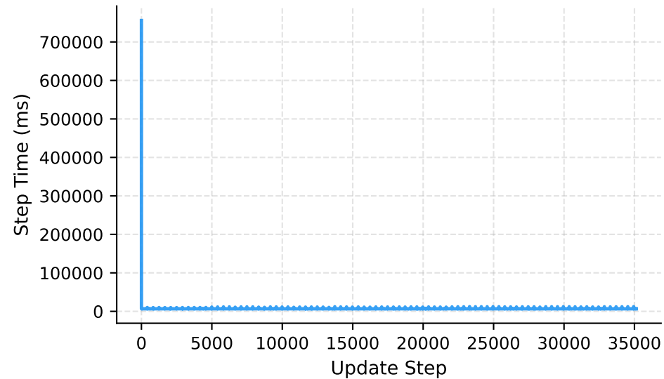
Step Duration
