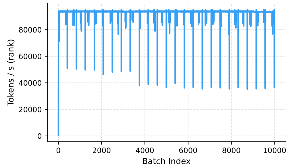
Per-Rank Throughput
