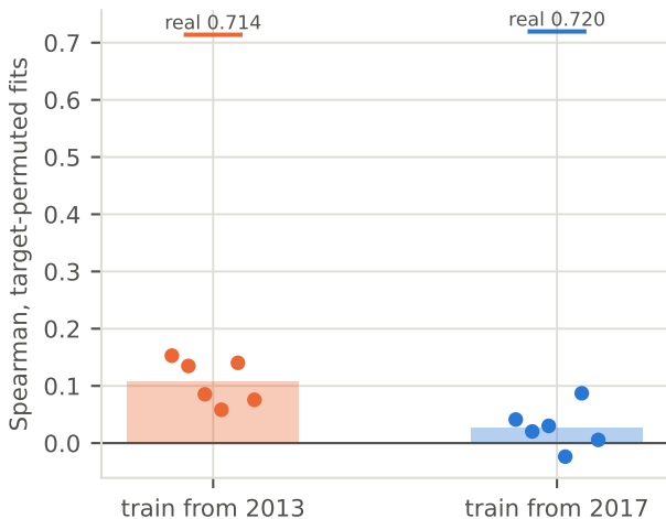
Points null control by training window
