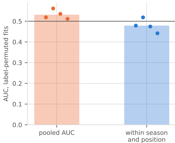
Injury null control by evaluation grain
