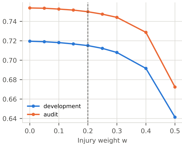
Spearman vs realized points
