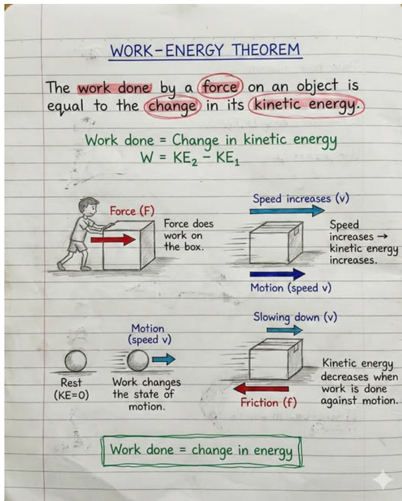
Figure 3: illustration on the work-energy theorem. Taken from edusphere academy.
