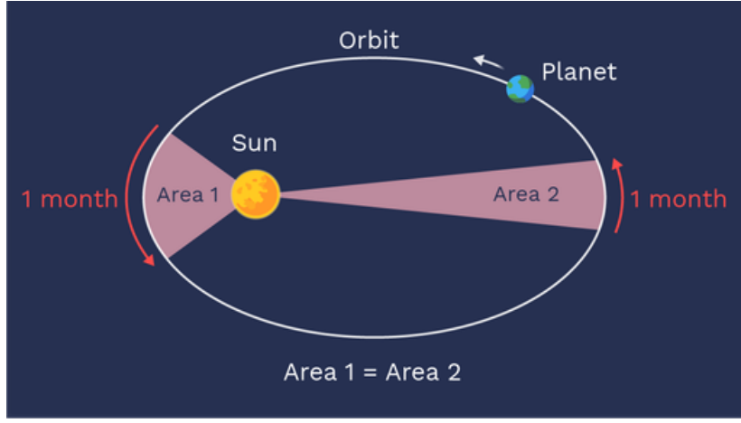
Figure 6: Kepler law is a consequence of angular momentum conservation. Indeed, for astral bodies, only the gravitational force (which is a central force) is applied. As a consequence of this conservation, the radius vector from the Sun to the planet sweeps out equal areas in equal times. This is Kepler's second law . Taken from here
