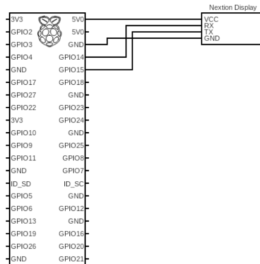
Figure 3.2: Eletric diagram of the Raspberry Pi and Nextion screen
