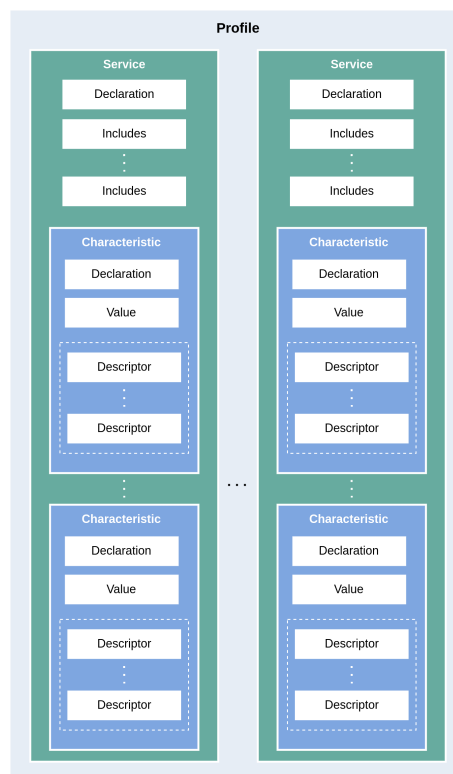
Figure 2.3: BLE GATT Hierarchical Architecture [13]
