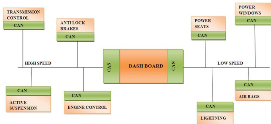
Figure 2.2: CAN Application Example [4]
