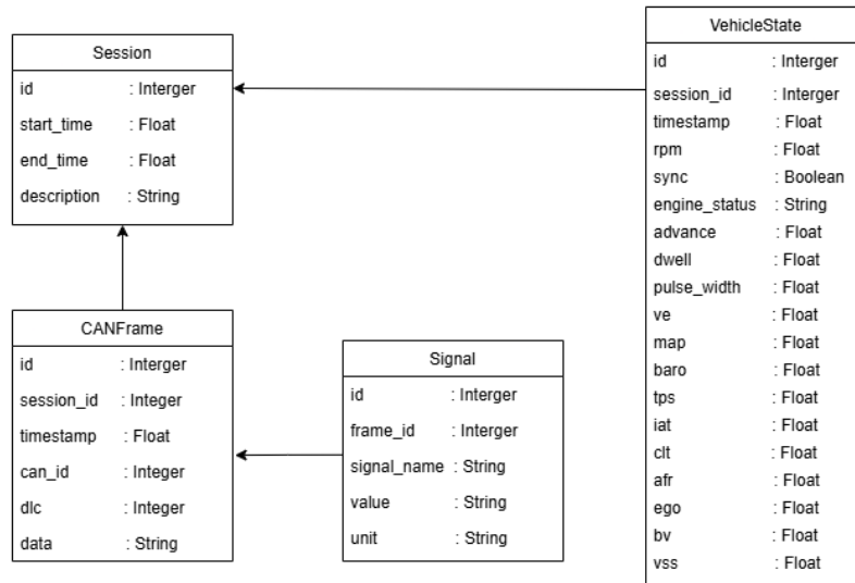
Figure 3.6: Database Diagram
