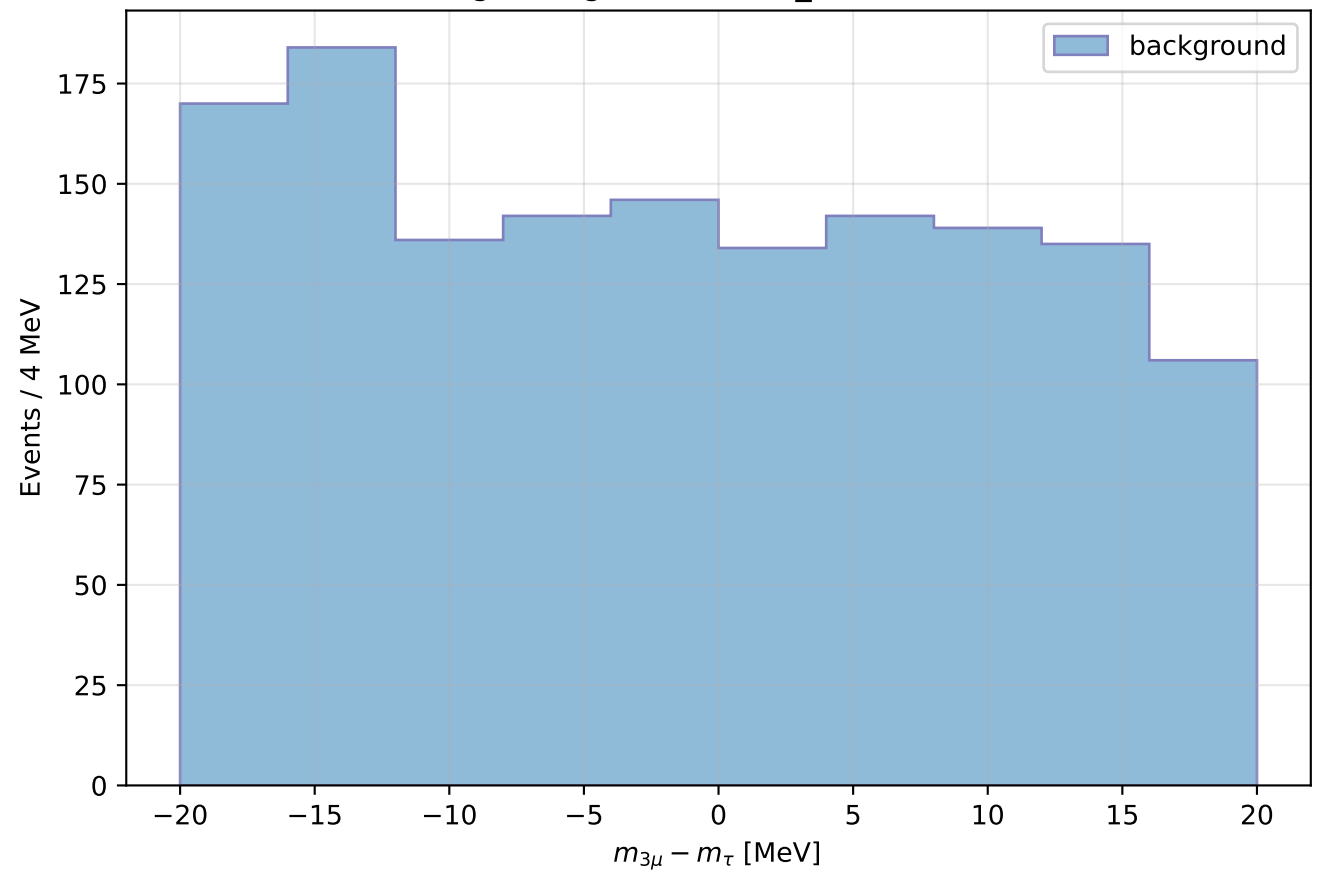
Signal region zoom (N_SR = 1434)
