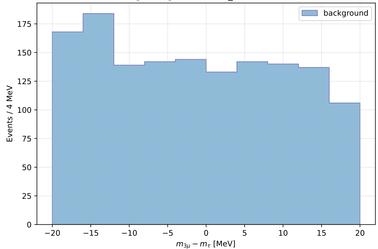
Signal region zoom (N_SR = 1435)
