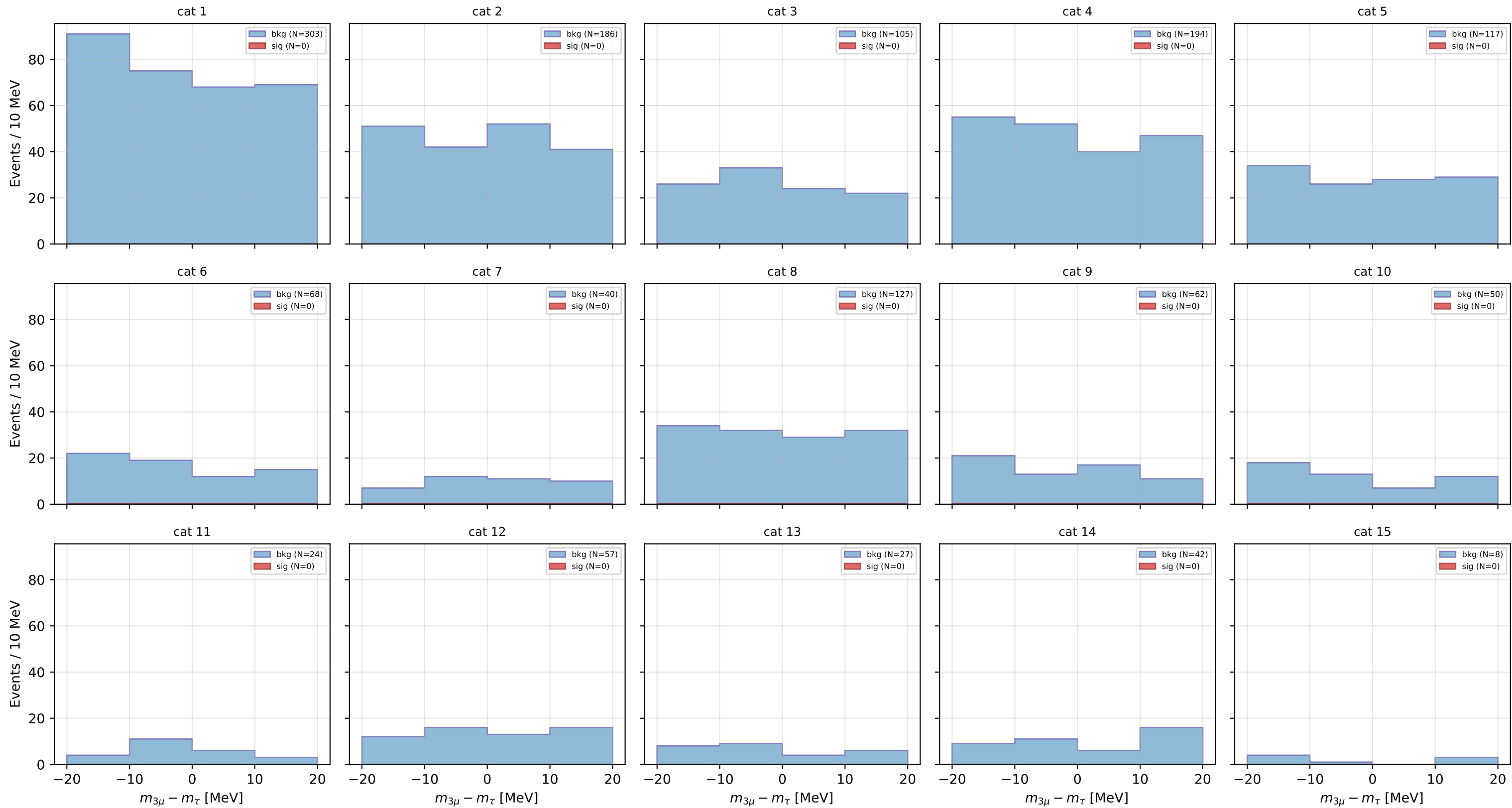
Toy per category: background (blue) + signal (red)
