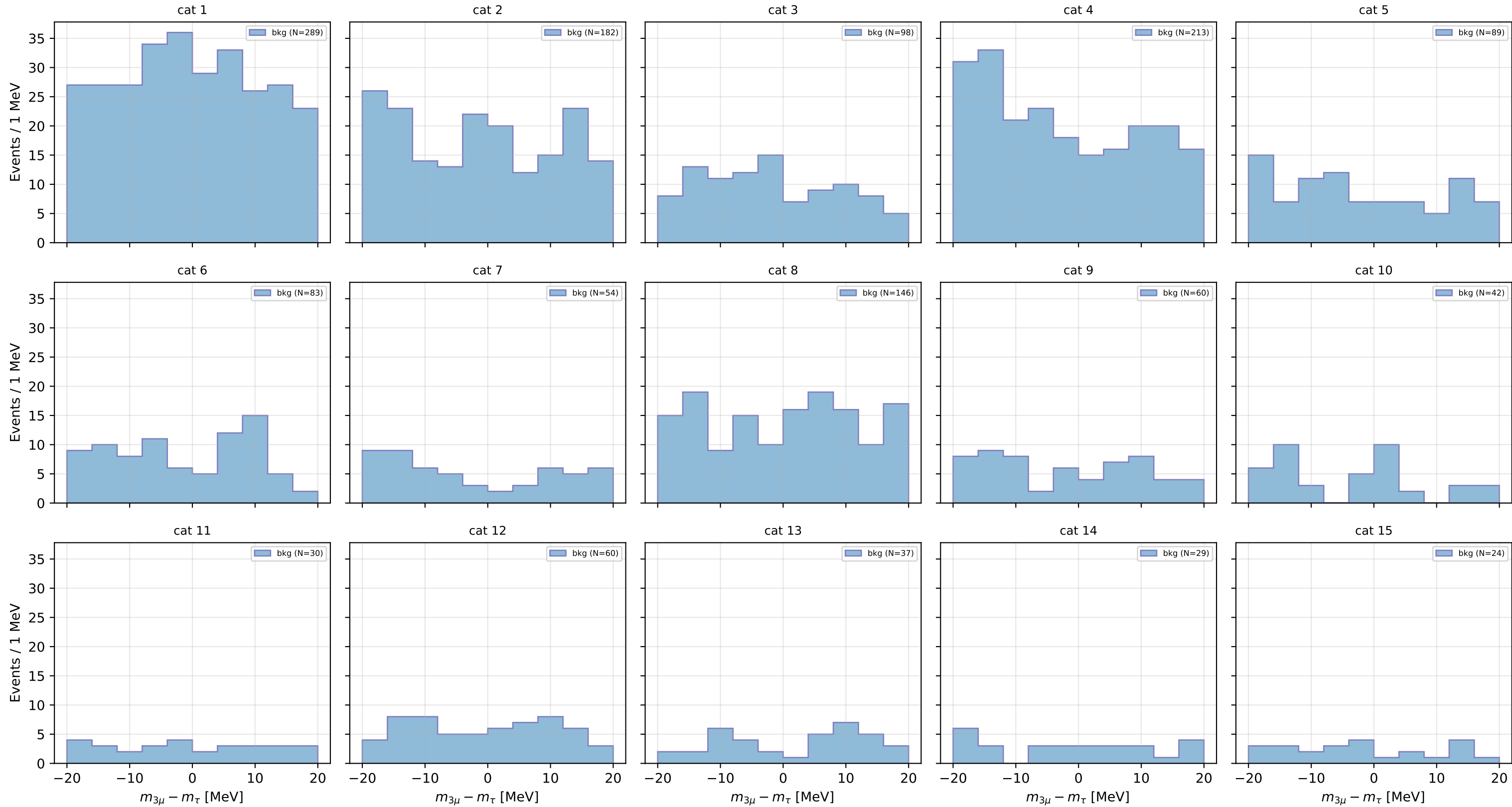
Toy per category (signal region zoom)
