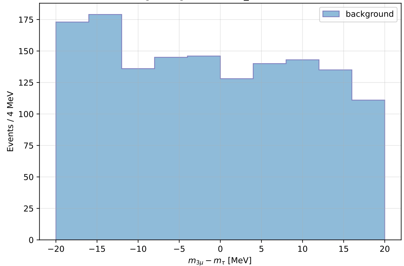
Signal region zoom (N_SR = 1476)
