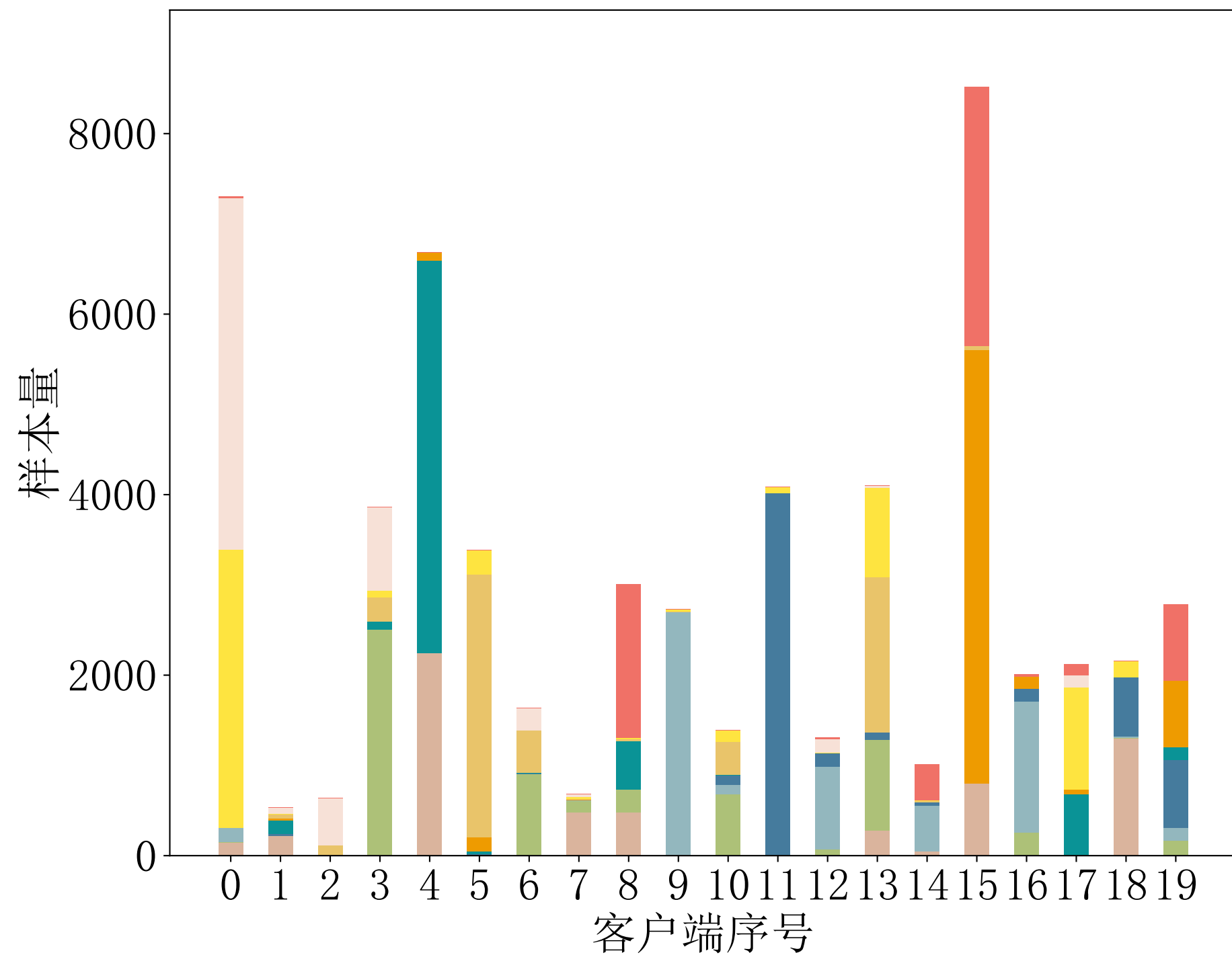
(a) Fashion-MNIST \alpha=0.1
