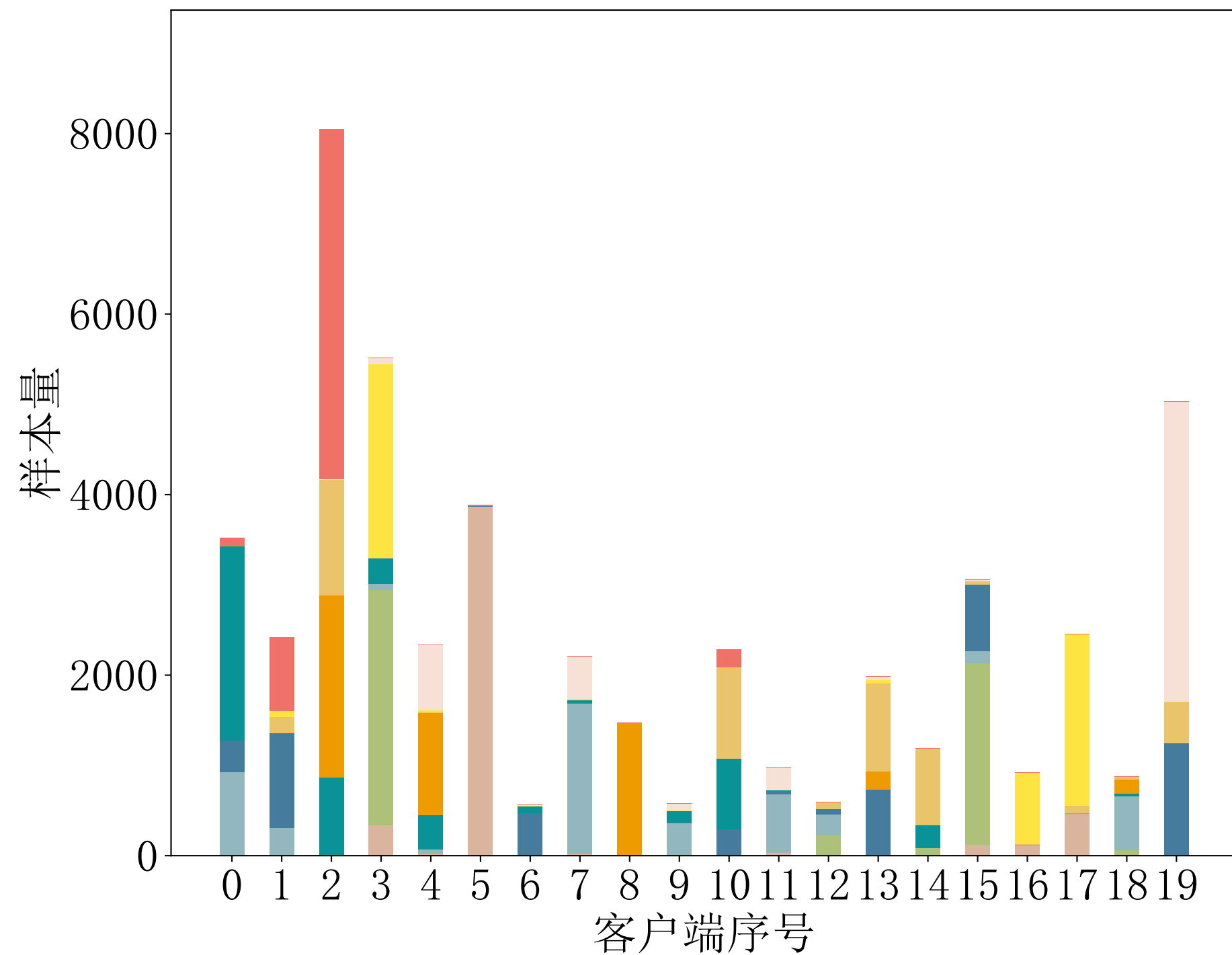
(b) CIFAR-10 \alpha=0.1
