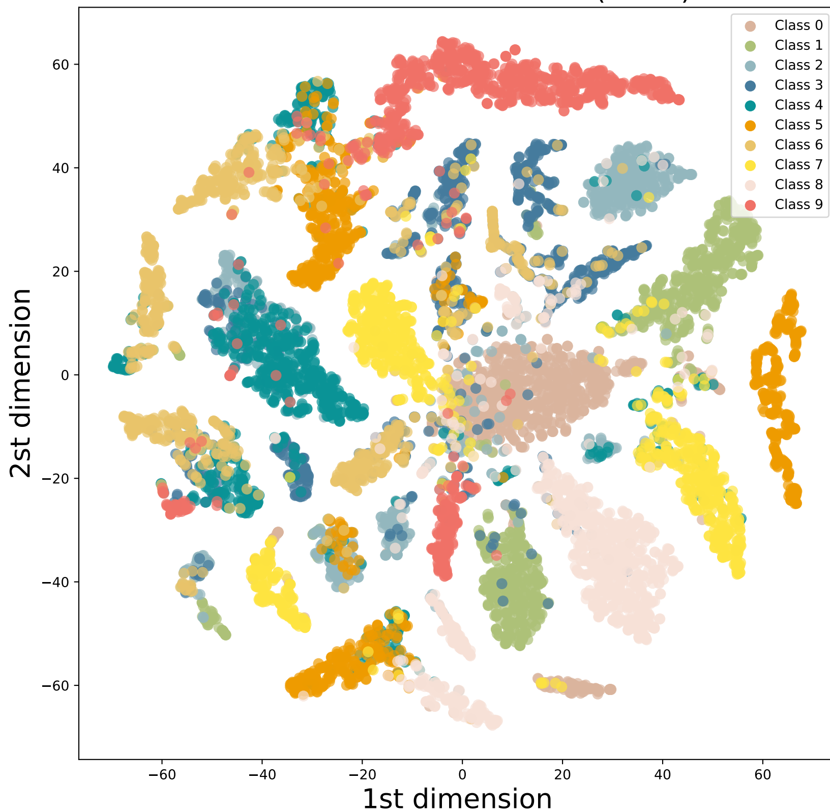
FedSC-Feature Distribution (t-SNE)
