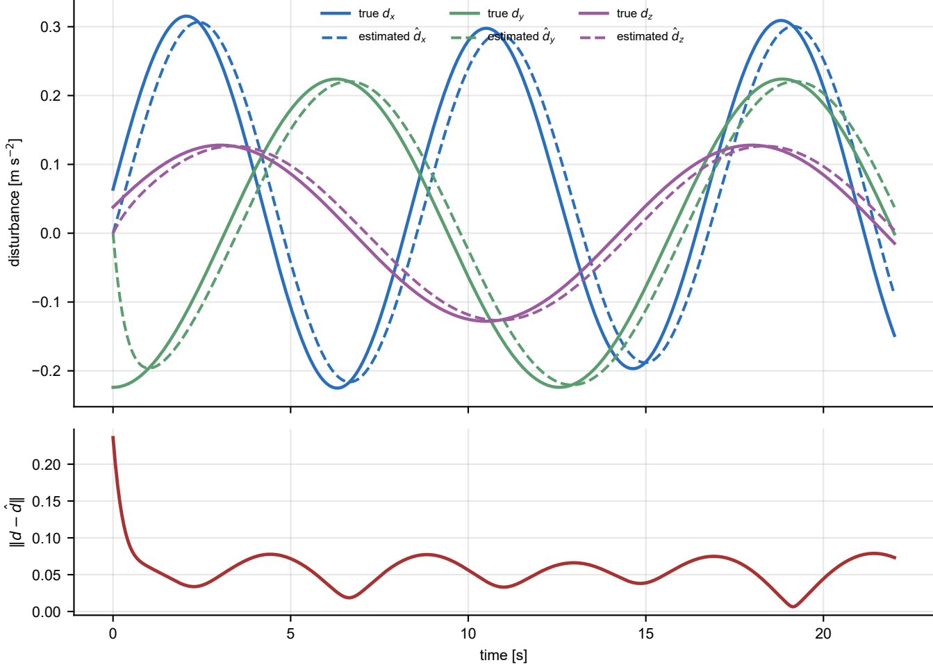
Disturbance-observer diagnostic under strong disturbance
