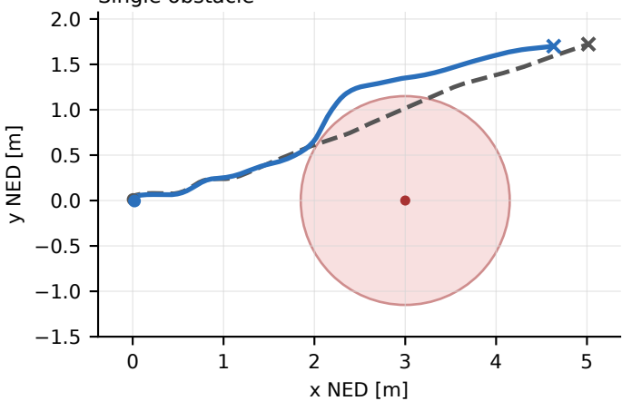
a Single obstacle
