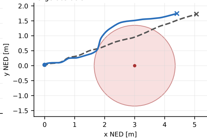
b Large obstacle
