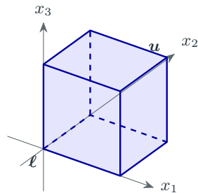
(g) Finite box ( d = 3 )
