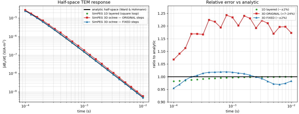
Figure 3: Before/after the fix. The original time-stepping (red) versus the fixed time-stepping (blue), the 1D layered solution (green), and the analytic (black). The fix moves the 3D response from +7–24 % to within \sim \pm 2\% .
