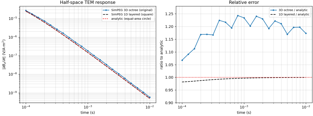
Figure 4: Localizing the discrepancy. Left: the half-space decay. Right: ratio to the closed-form analytic. The SimPEG 1D layered solution (black dashed) tracks the analytic to within \sim 2\% ; the original 3D octree run (blue) is 7–24% high and jagged.
