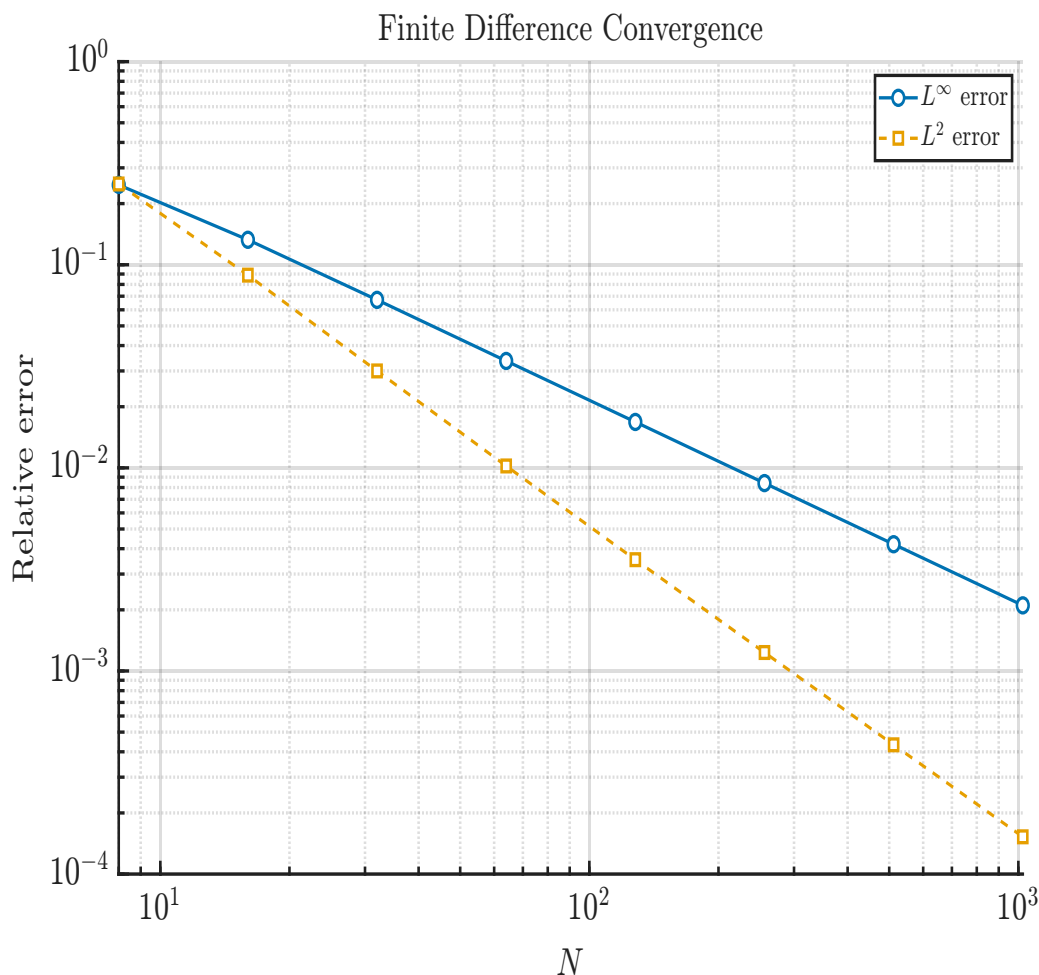
Figure 2: Comparison of the exact derivative of f(x) = e^{\sin x} with the finite difference approximation.
