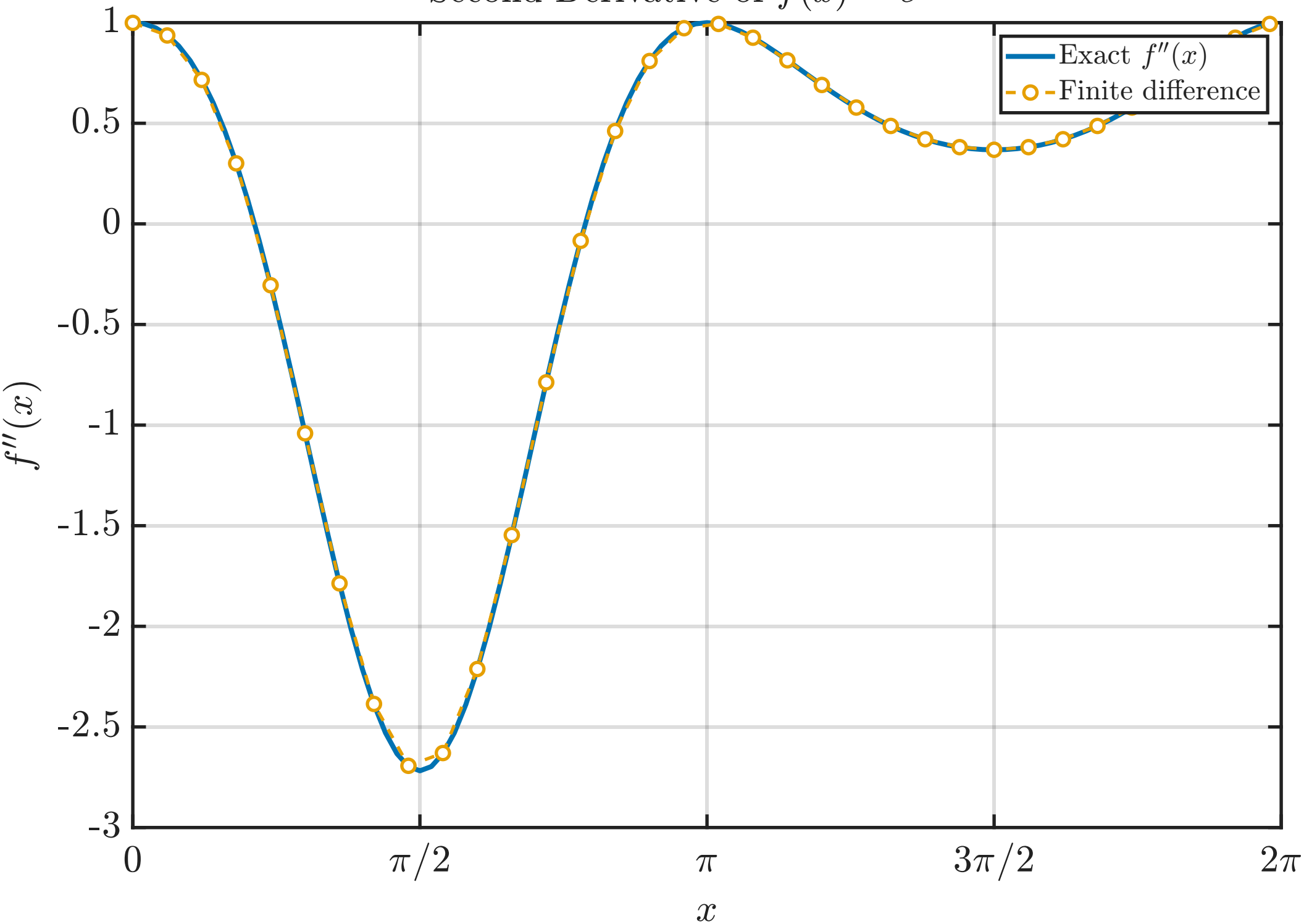
Second Derivative of f(x) = e^{\sin(x)}
