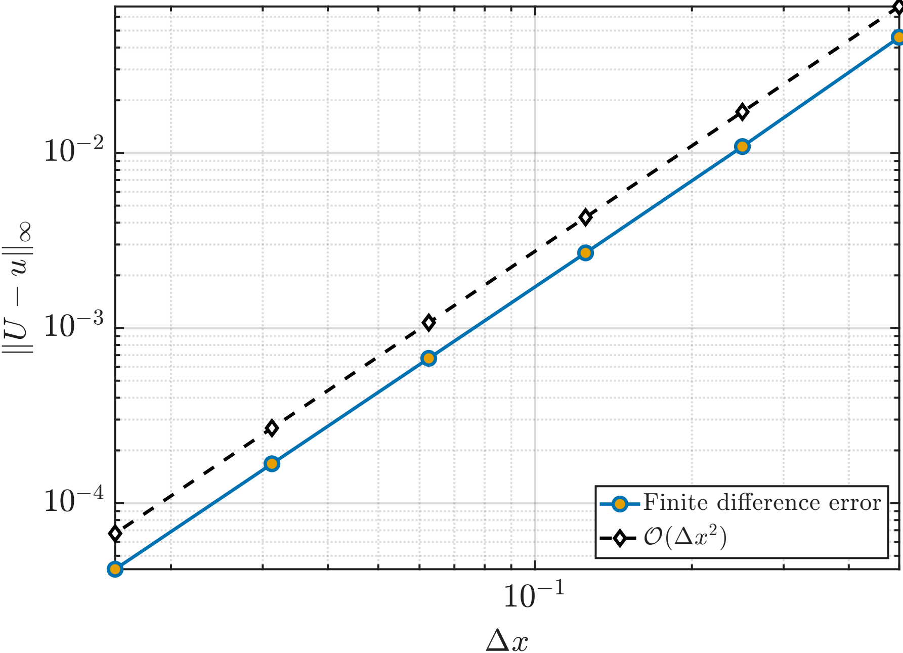
Convergence Plot
