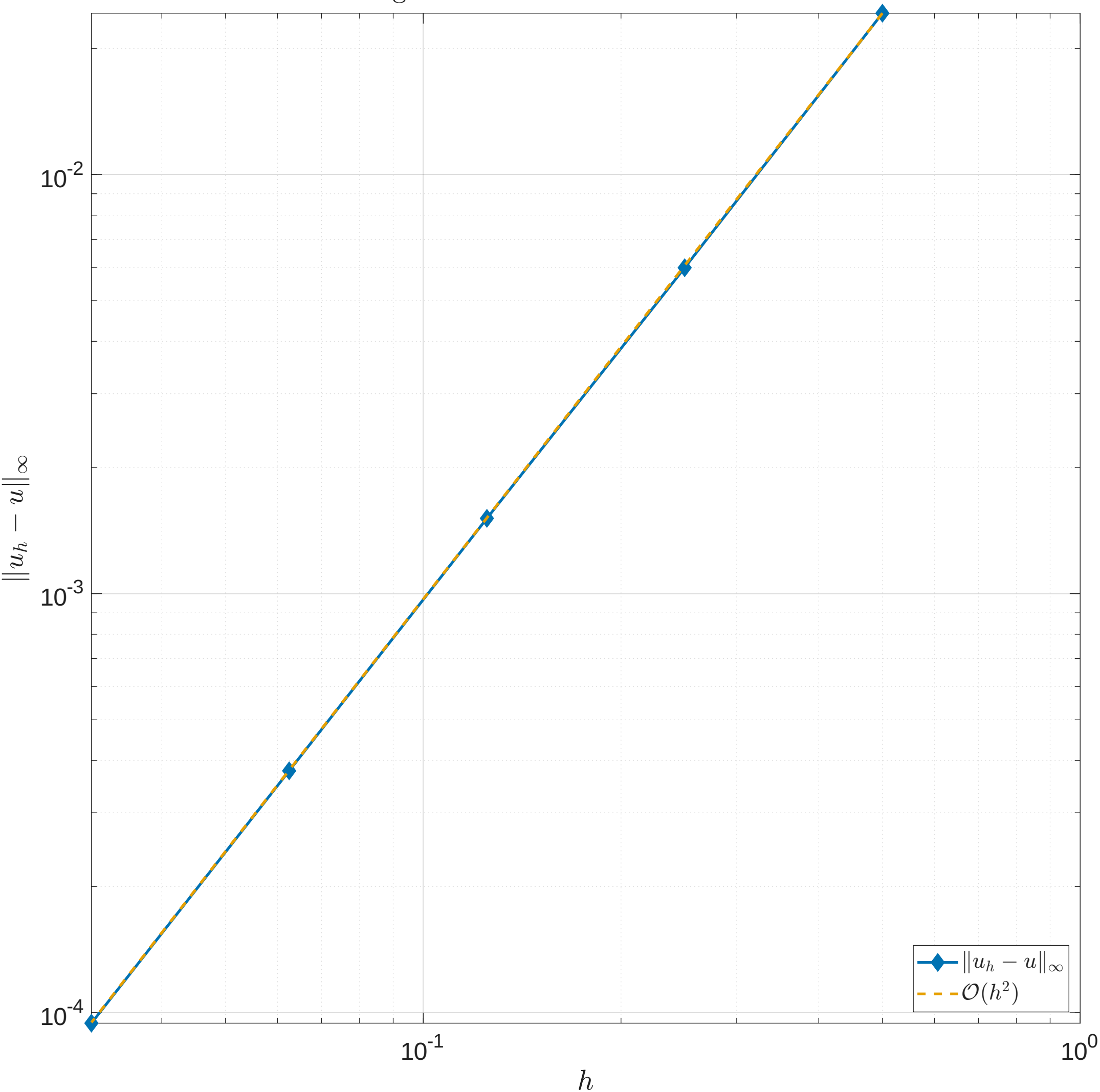
Convergence of the Finite Difference Solution
