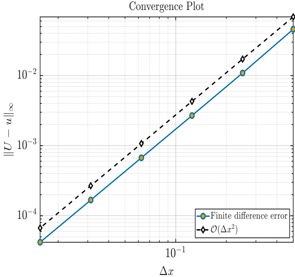
Figure 5: Finite difference error plotted alongside \mathcal{O}(\Delta x^2) with log-log scale
