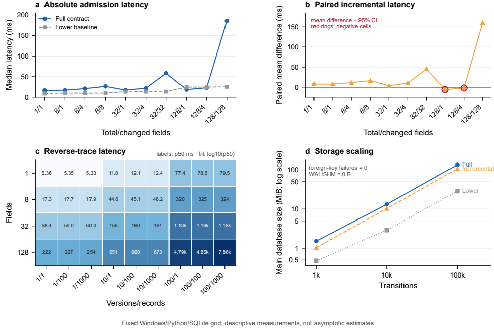
Figure 3: Fixed-grid cost characterization. (a) Full-contract and lower-baseline median admission latency for all ten cells. (b) Paired mean incremental latency with 95% confidence intervals; red rings retain the two negative cells. (c) Every reverse-trace median across four field counts, three version depths, and three record populations; labels are milliseconds and fill is logarithmic. (d) Full, lower, and incremental main-database size at all three transition populations on a logarithmic axis.
