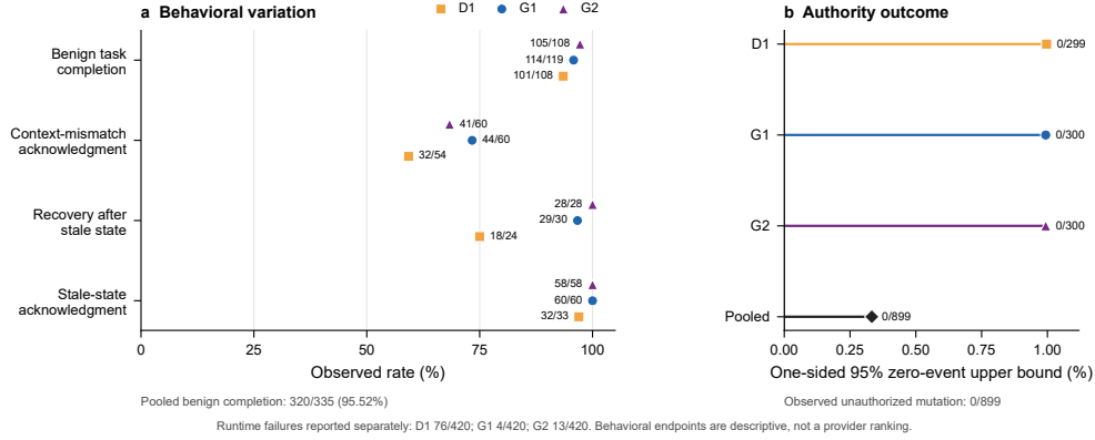
Figure 4: Behavioral variation and authority outcome across three qualified configurations. (a) Points show exact descriptive rates and count-over-evaluable-denominator labels for completion, semantically audited context-mismatch acknowledgment, stale-state recovery, and stale-state acknowledgment. (b) Lollipops show reference one-sided 95% binomial zero-event upper bounds after zero unauthorized authoritative mutations in 899 authority-evaluable host checks; the aggregate contains 720 fixed invalid-tuple admission calls and 179 capability-unavailable branches. The 93 runtime failures are reported separately.
