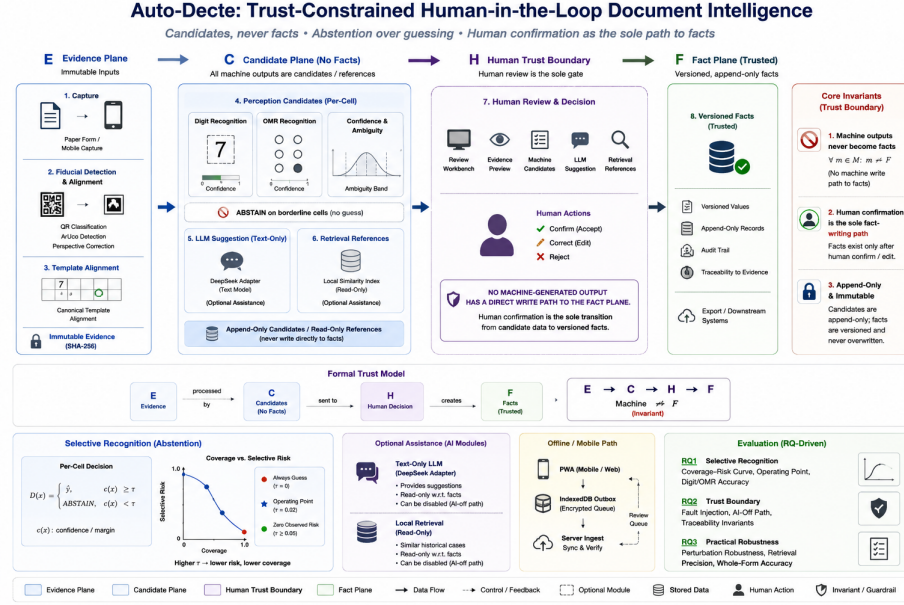
Fig. 1. Trust-constrained architecture of Auto-Decte. Evidence is transformed into machine-generated candidates or read-only references, while the human trust boundary is the sole transition from candidate data to versioned facts. Recognition, LLM suggestions, and retrieval have no direct write path to the fact plane.
