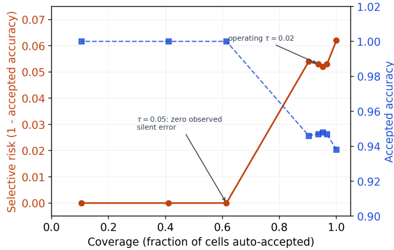
Fig. 2. Coverage vs selective risk over the abstention threshold. Increasing \tau lowers coverage but drives the observed selective risk to zero on the controlled benchmark; the operating point \tau=0.02 is marked.
