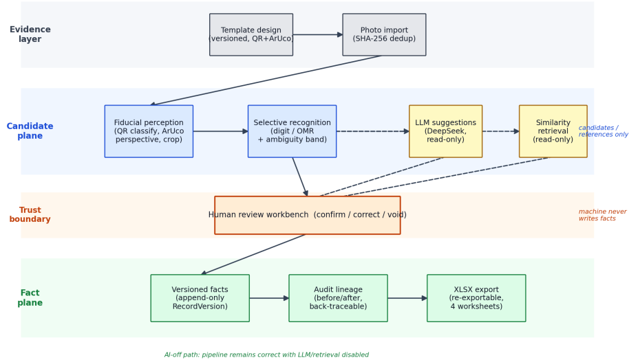
Fig. 1. Trust-constrained architecture of Auto-Decte. Evidence is transformed into machine-generated candidates or read-only references, while the human trust boundary is the sole transition from candidate data to versioned facts. Recognition, LLM suggestions, and retrieval have no direct write path to the fact plane.
