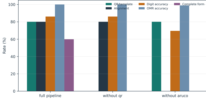
Figure 6: Whole-form component-suppression analysis. Removing a component required by the endpoint forces complete success to zero; field metrics show the additional recognition effect of missing alignment.
