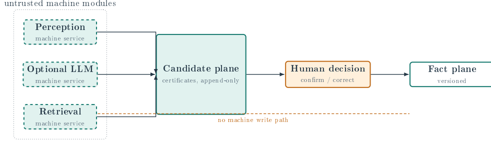
Figure 1: Trust model. Dashed machine components terminate at append-only candidates or read-only references; an attributable human decision is the only exposed path to a versioned fact. The diagram was drafted with the assistance of a generative-AI tool (DeepSeek Harness) and verified by the author for architectural accuracy.
