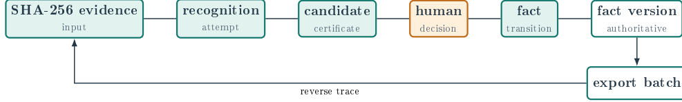
Figure 3: Evidence lineage from content-addressed input to export. Every arrow represents a persisted identifier used by the reverse-trace check; each fact field rebuilds evidence–certificate–decision–transition from the database. The diagram was drafted with the assistance of a generative-AI tool (DeepSeek Harness) and verified by the author for architectural accuracy.
