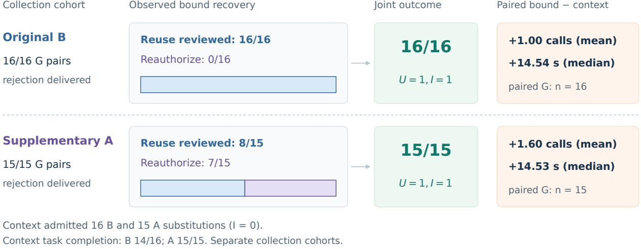
Figure 3: Accountable recovery and paired execution costs at the standardized G boundary. Original B contributes 16 delivered G-bound mismatch episodes and supplementary A contributes 15; all end with U = 1, I = 1 . B uses reviewed-candidate reuse throughout; supplementary A uses reuse in eight cases and reauthorization in seven. Calls are means and seconds are medians of bound-minus-context differences across the corresponding G task pairs, measured over the complete suffix.
