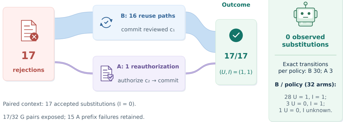
Figure S3: Original observed paths after standardized mismatch feedback. All 17 exposed G-bound continuations recover with (U, I) = (1, 1) : B reuses the reviewed candidate in 16 cases, and A reauthorizes the handoff candidate in one. The separate N panel retains agent-managed preview outcomes and unknown coverage. The figure reports observed paths, not the frequency of naturally occurring substitutions.
