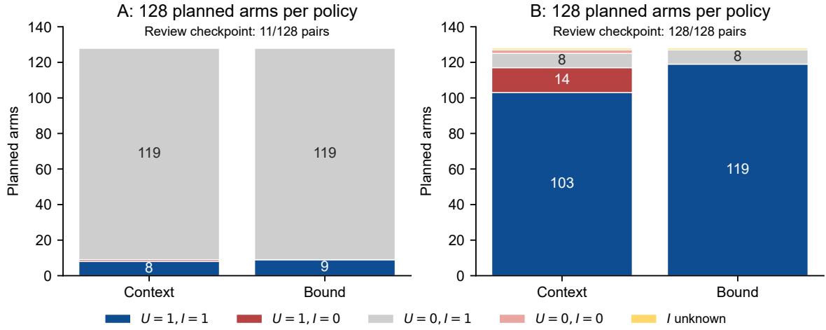
Figure S2: Original planned-ledger utility and integrity. Each policy/deployment column contains 128 arms. The large U=0, I=1 component in A reflects covered state with provider failures, predominantly before review. Small joint cells and both unknowns remain explicit in the main joint-outcome table and the complete table below.
