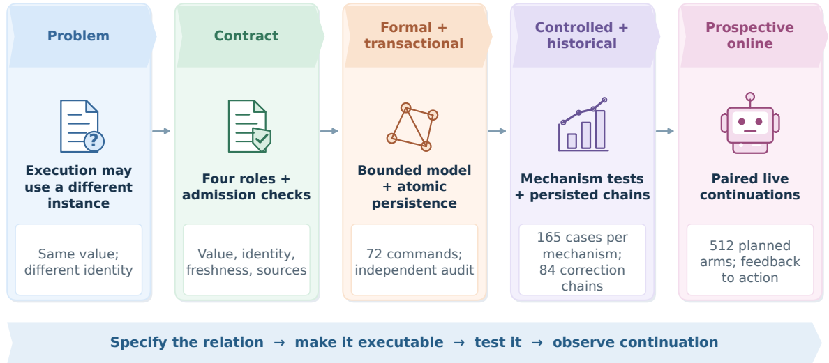
Figure S1: Evidence chain for trustworthy corrected execution. Distinct layers define continuity, make it executable, validate persistence and integration, then observe live agent continuation. Counts retain separate units: bounded commands, cases per mechanism, archived correction chains and planned paired trajectories.
