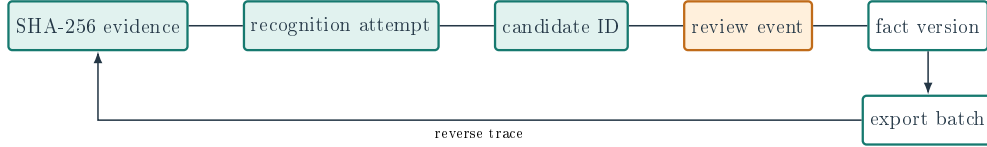
Figure 3: Evidence lineage from content-addressed input to export. Every arrow represents a persisted identifier used by the reverse-trace check.
