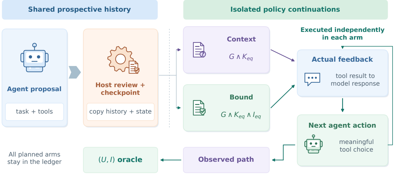
Figure 2: Paired online intervention after a shared prospective review. The visible conversation and persisted checkpoint are copied into isolated policy arms. The only execution-rule difference is I_{eq} . Actual tool feedback enters the next sampled agent decision, whose actions and terminal state are independently audited. The standardized G handoff supplies an index request; N instead leaves refreshed-preview management to the agent.
